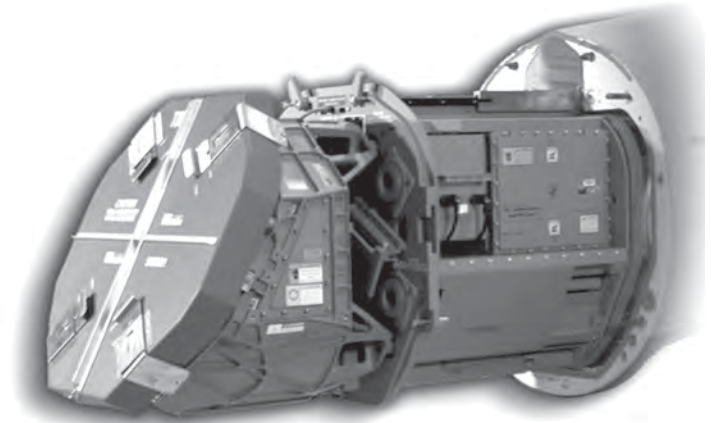
The APG-79 AESA radar system is an upgrade to the F/A-18 E/F Super Hornet and replaces the APG-73 mechanically scanned array radar.
